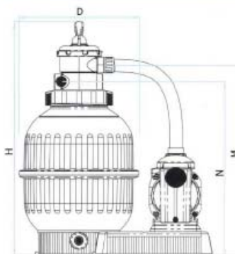
Filteranlage "Cantabric Top" Top-mount monobloc
